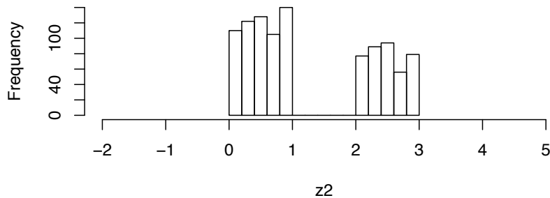
Histogram of z_2
