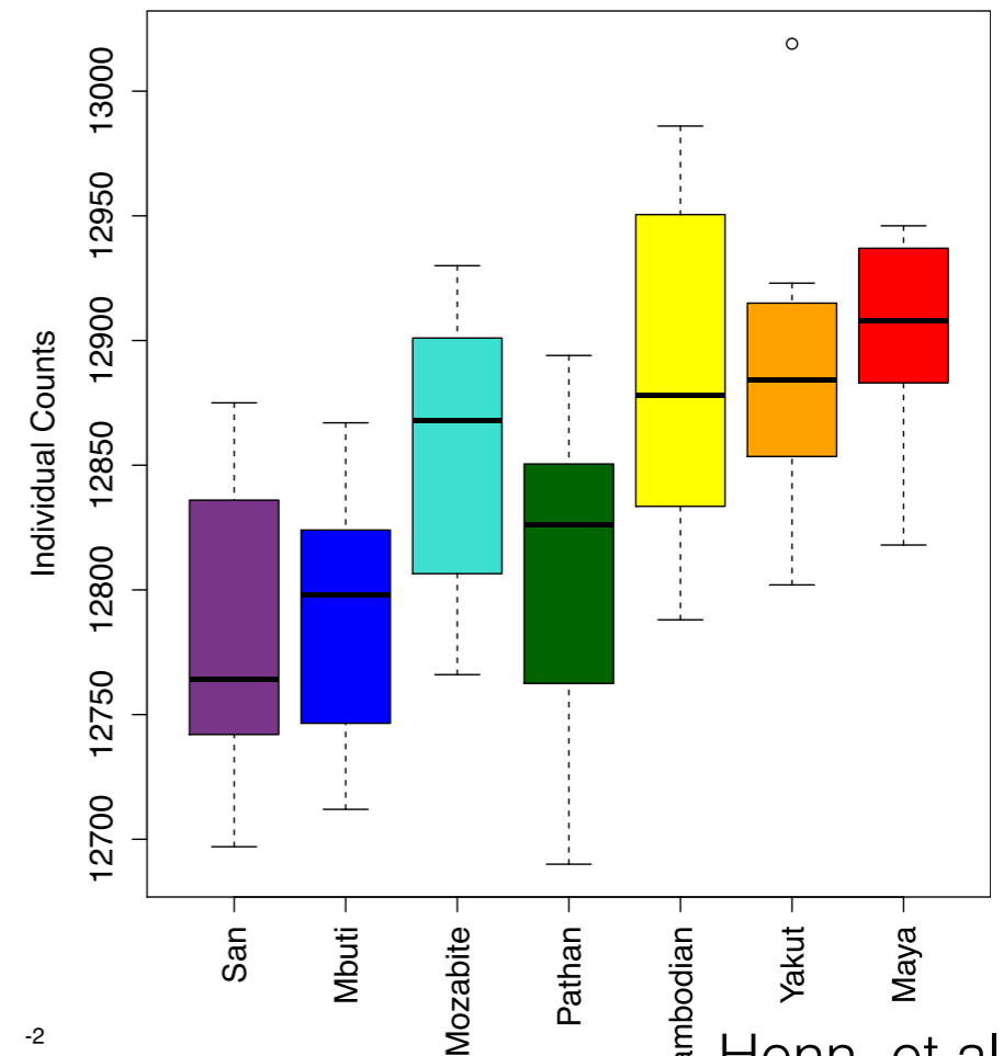
Individual number of deleterious counts
