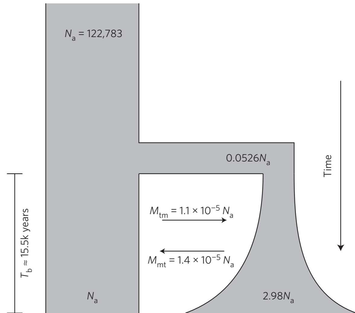
Figure 2 | Estimated demographic history of maize and teosinte. Parameter estimates for a basic bottleneck model of maize domestication. See Methods for details.
