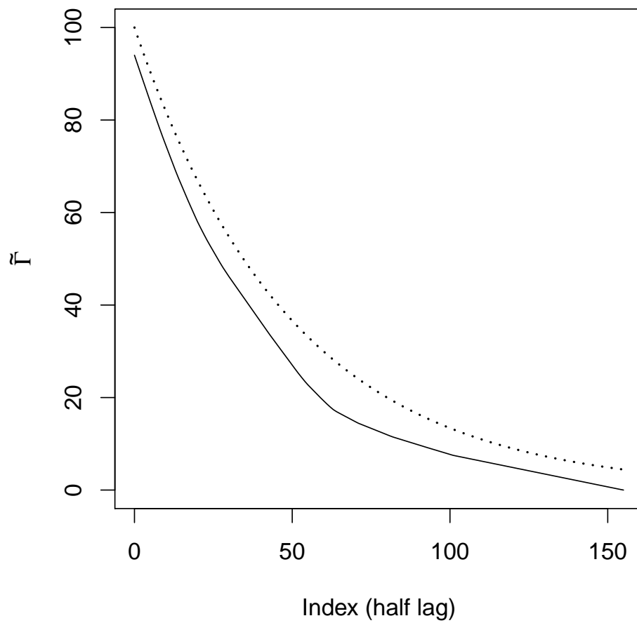
Figure 1.6: Big Gamma Plot for AR(1) Example. Solid line: initial convex sequence estimator of (1.10.3). Dotted line: theoretical value.
