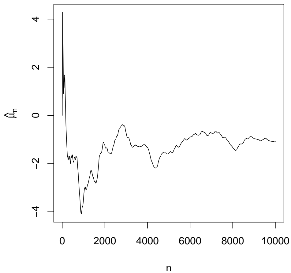
Figure 1.2: Running Averages Plot for AR(1) Example.
