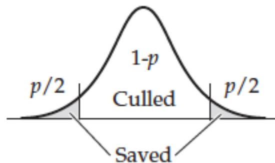
Disruptive selection
