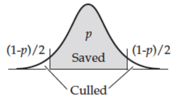
Stabilizing selection
