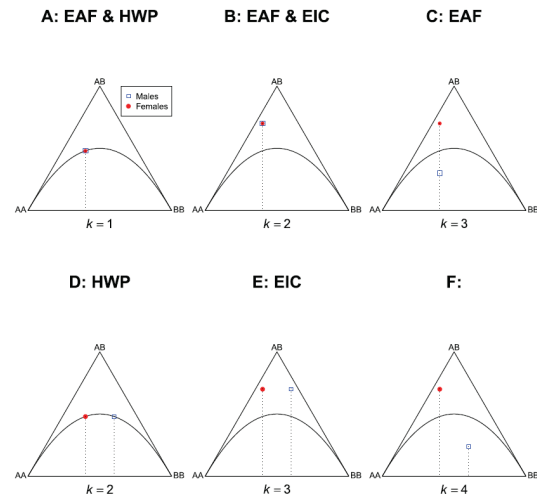
FIGURE 2 Ternary diagrams for male and female genotype frequencies Notes: (A) HWP and EAF. (B) Equality of inbreeding coefficients, EAF, and both sexes out of HWP. (C) Unequal inbreeding coefficients, both sexes out of equilibrium but with equal allele frequencies. (D) Both sexes in HWP but with different allele frequencies. (E) Each sex out of equilibrium with identical inbreeding coefficients and different allele frequencies. (F) Both sexes out of equilibrium, with different inbreeding coefficients and different allele frequencies. The number of free parameters k is given below the basis of each scenario.
